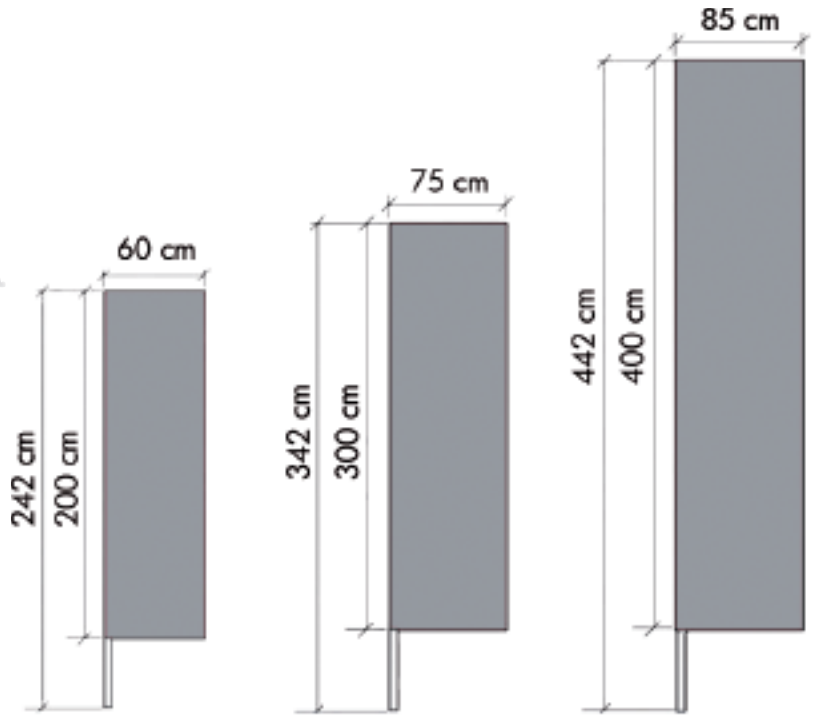
S Pole size 2,42 m M Pole size 3,42 m L Pole size 4,42 m
